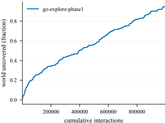
Cumulative coverage -- EpicChase4-90@6
