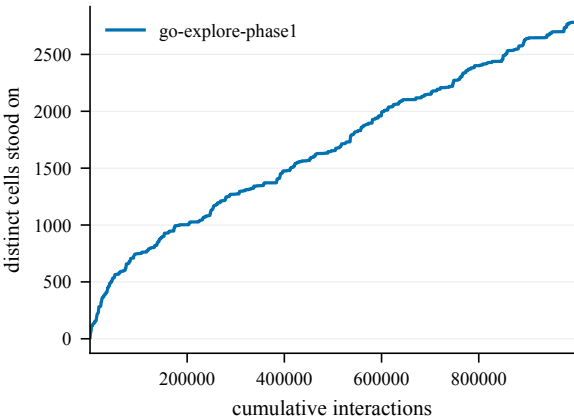
States discovered -- EpicChase4-90@6
