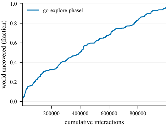
Cumulative coverage -- EpicChase4-90@8
