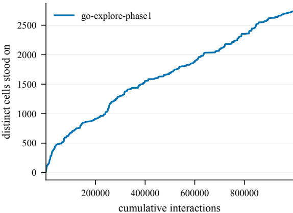
States discovered -- EpicChase4-90@9
