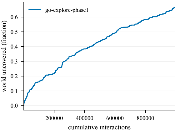
Cumulative coverage -- EpicChase6-110@10
