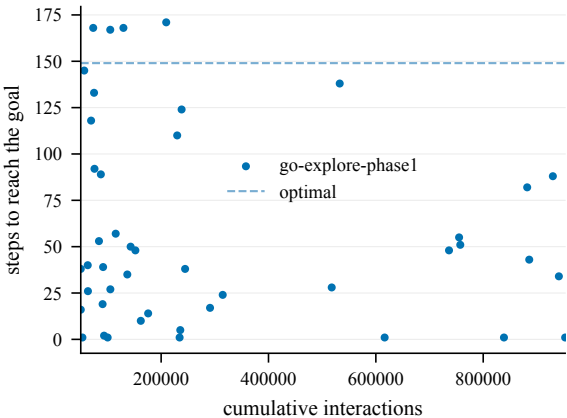
Steps to goal (train) -- EpicChase6-110@10
