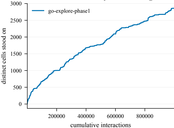
States discovered -- EpicChase6-110@14
