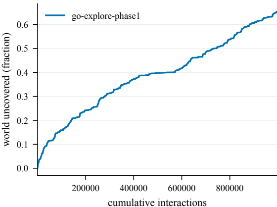
Cumulative coverage -- EpicChase6-110@16
