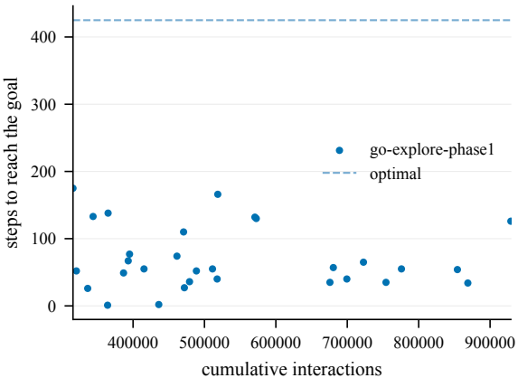
Steps to goal (train) -- EpicChase6-110@16
