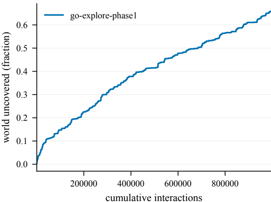
Cumulative coverage -- EpicChase6-110@18
