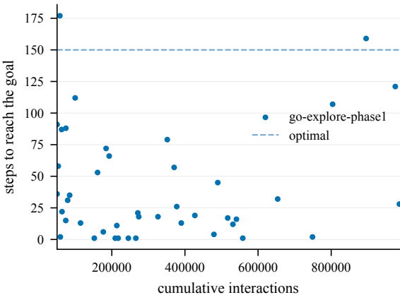
Steps to goal (train) -- EpicChase6-110@2
