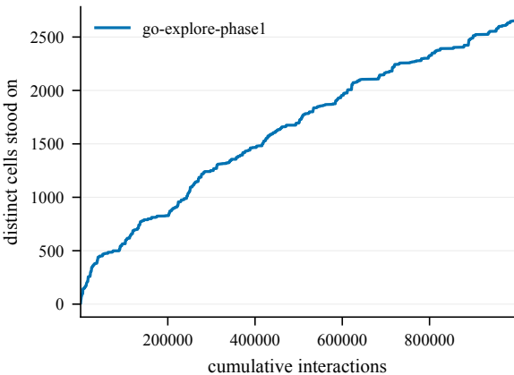
States discovered -- EpicChase6-110@2
