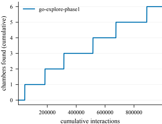
Chambers -- EpicChase6-110@23
