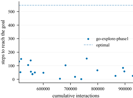
Steps to goal (train) -- EpicChase6-110@24
