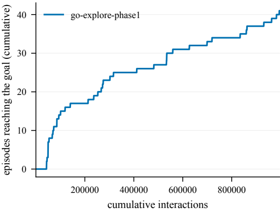
Goal reached -- EpicChase6-110@28
