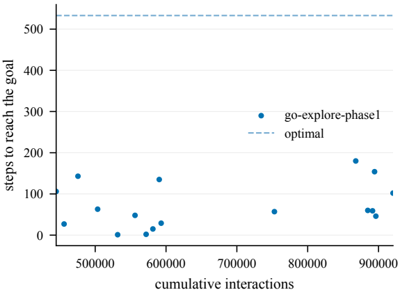
Steps to goal (train) -- EpicChase6-110@3
