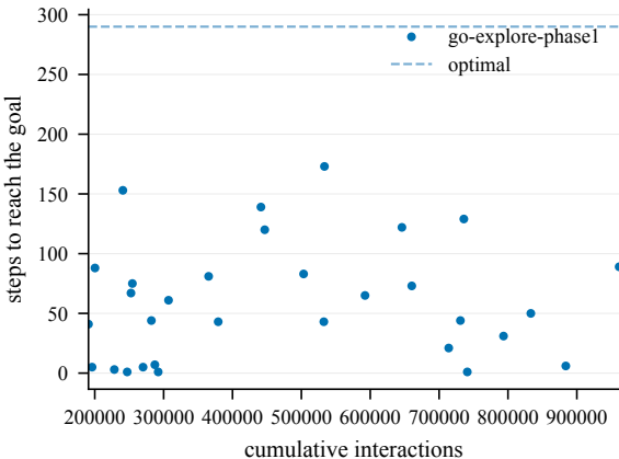
Steps to goal (train) -- EpicChase6-110@5
