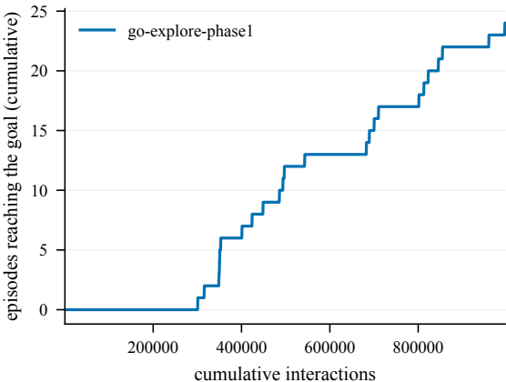
Goal reached -- EpicChase6-110@6
