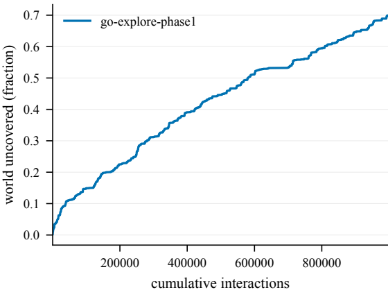
Cumulative coverage -- EpicChase6-110@6
