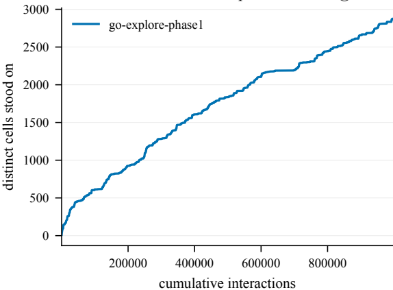
States discovered -- EpicChase6-110@6
