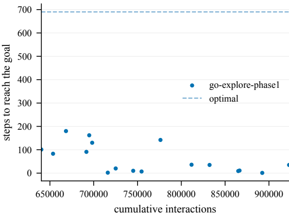
Steps to goal (train) -- EpicChase6-110@9
