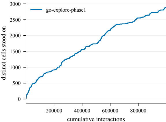
States discovered -- EpicChase6-110@9
