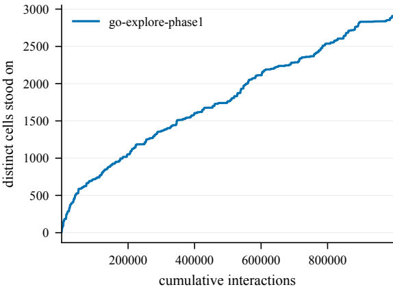
States discovered -- EpicChase8-120@10
