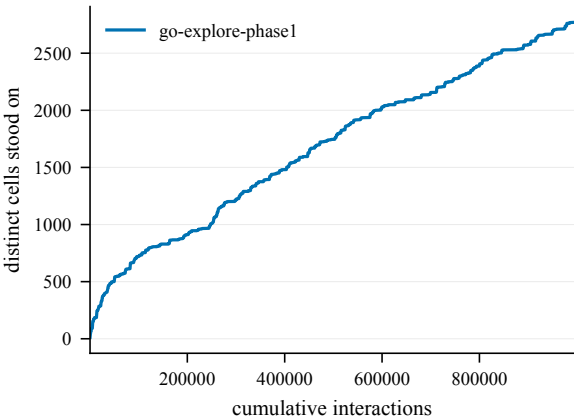
States discovered -- EpicChase8-120@11
