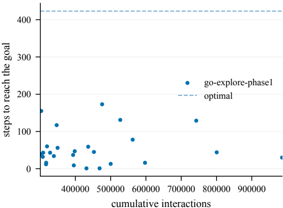
Steps to goal (train) -- EpicChase8-120@12
