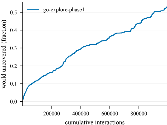
Cumulative coverage -- EpicChase8-120@13
