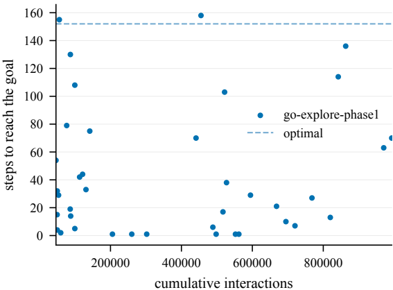
Steps to goal (train) -- EpicChase8-120@13
