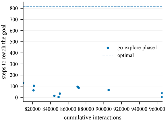
Steps to goal (train) -- EpicChase8-120@14
