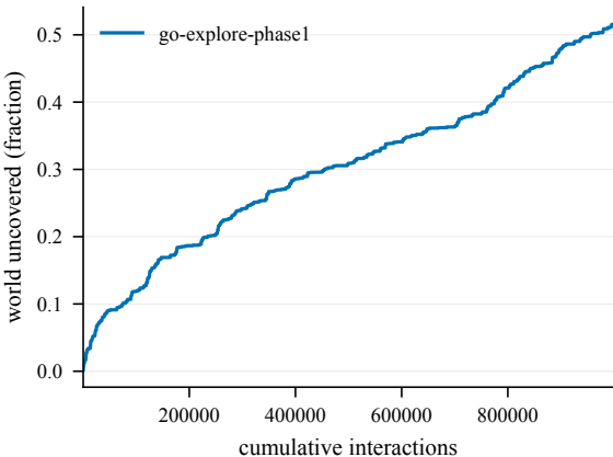
Cumulative coverage -- EpicChase8-120@16
