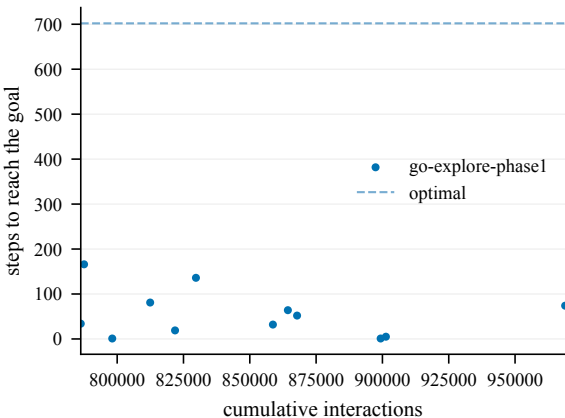
Steps to goal (train) -- EpicChase8-120@16
