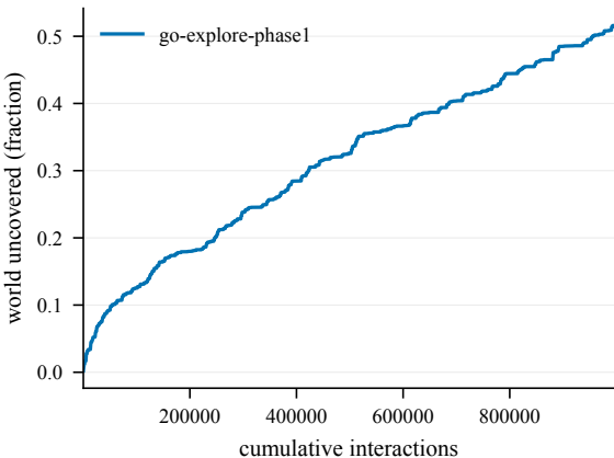
Cumulative coverage -- EpicChase8-120@17
