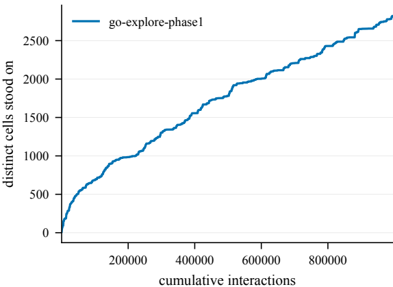
States discovered -- EpicChase8-120@17
