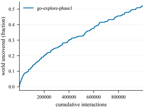
Cumulative coverage -- EpicChase8-120@2
