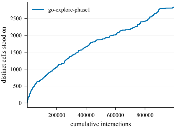
States discovered -- EpicChase8-120@20
