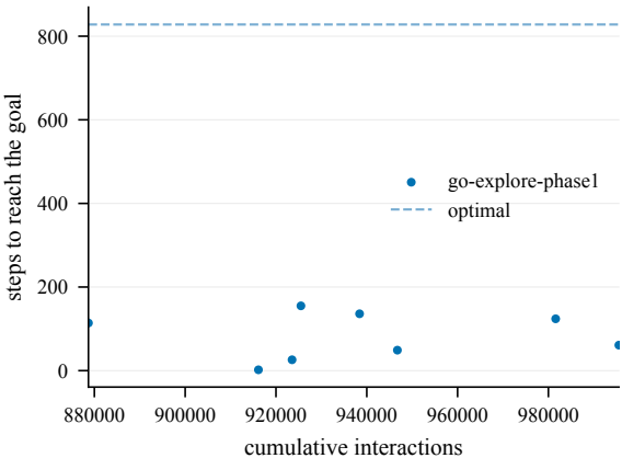
Steps to goal (train) -- EpicChase8-120@21
