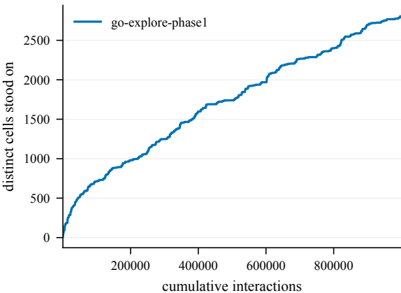
States discovered -- EpicChase8-120@21
