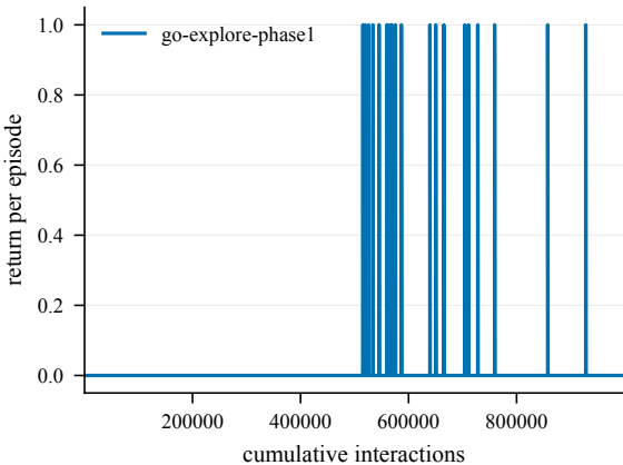
Return -- EpicChase8-120@22
