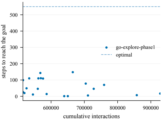
Steps to goal (train) -- EpicChase8-120@22
