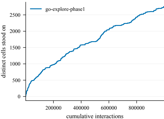
States discovered -- EpicChase8-120@24
