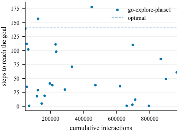
Steps to goal (train) -- EpicChase8-120@25
