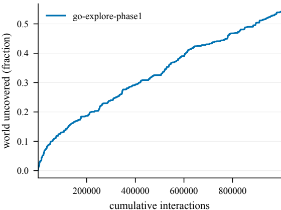
Cumulative coverage -- EpicChase8-120@26
