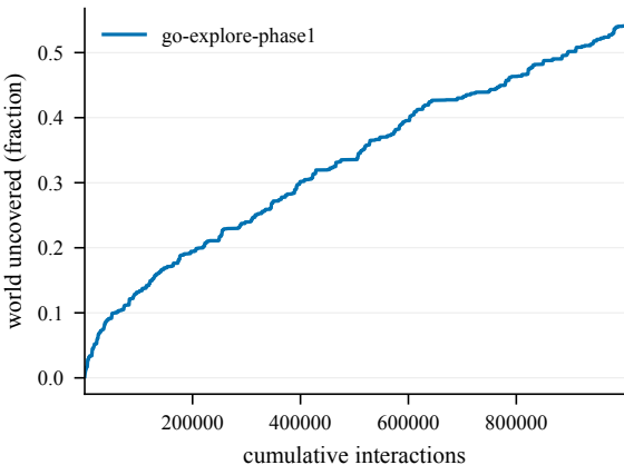
Cumulative coverage -- EpicChase8-120@27
