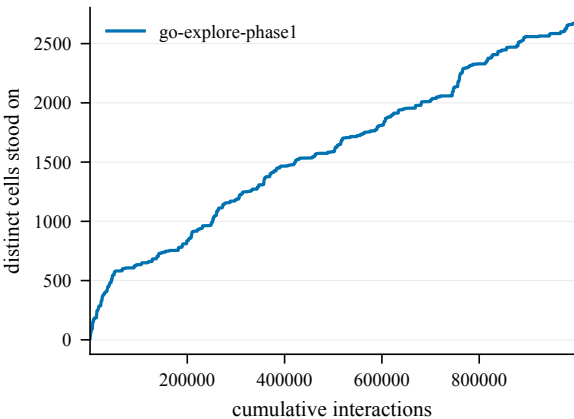
States discovered -- EpicChase8-120@28
