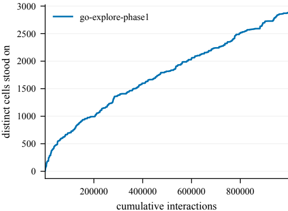
States discovered -- EpicChase8-120@29
