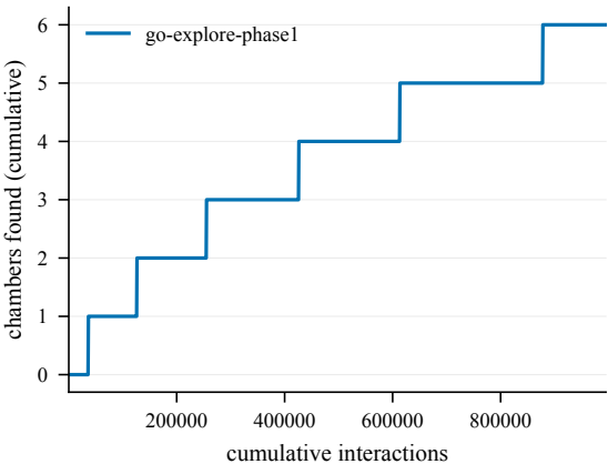
Chambers -- EpicChase8-120@3
