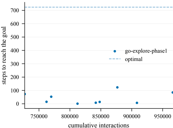
Steps to goal (train) -- EpicChase8-120@4
