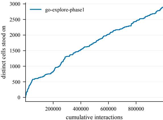
States discovered -- EpicChase8-120@5
