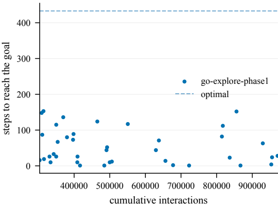
Steps to goal (train) -- EpicChase8-120@7
