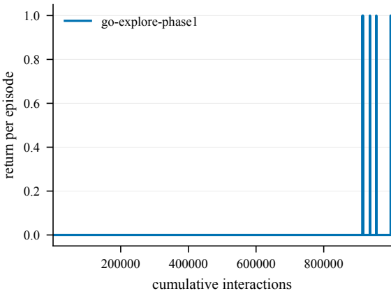
Return -- EpicChase8-120@9
