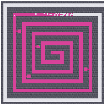
Go-Explore
